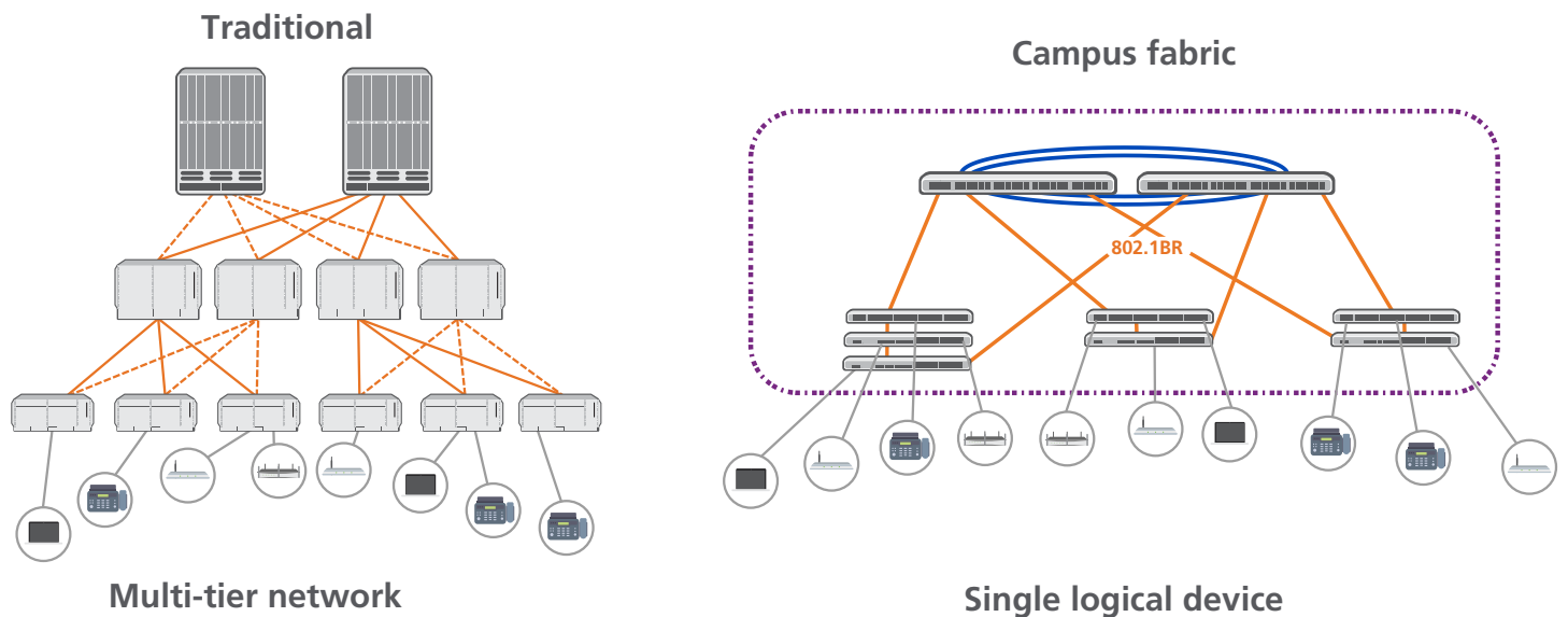
Figure 2: The RUCKUS campus fabric architecture versus a traditional multi-tier campus network.
