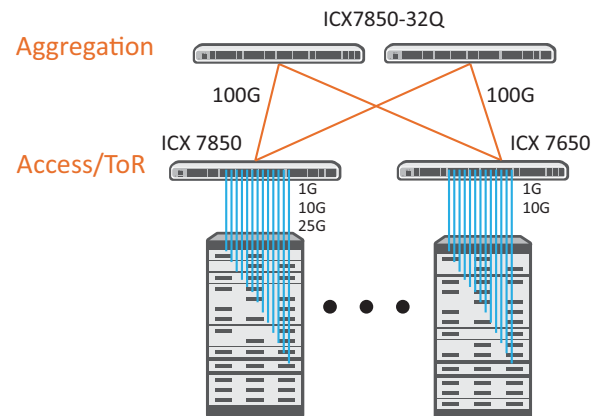
Figure 6: Data center top-of-the-rack connectivity.
