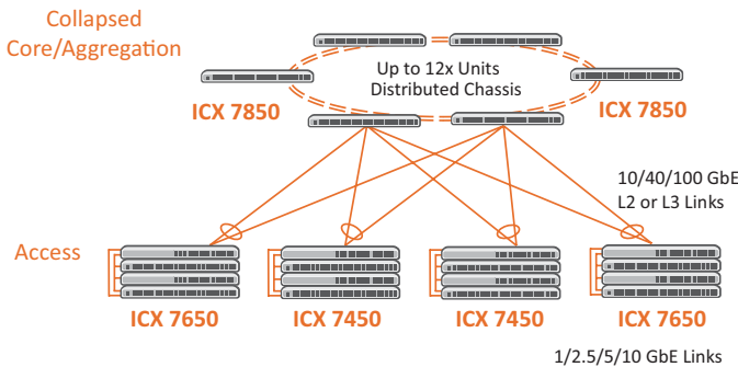
Figure 4: Two-tier campus network.
