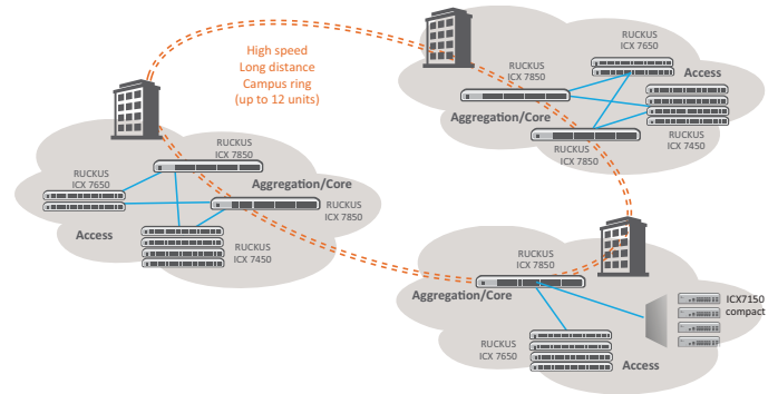
Figure 5: Distributed two-tier campus network.
