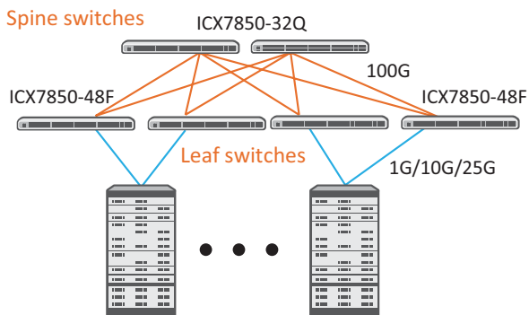
Figure 7: ICX 7850 spine-leaf solution.
